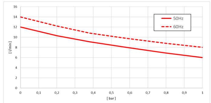
NOTE: Curves refers to 1013mbar (abs.) pression and 20°C temp. (tolerance ±10%).
