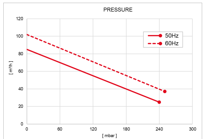
Curves refer to 1013mbar (Abs.) pression and 20°C temperature (tolerance ±10%)
