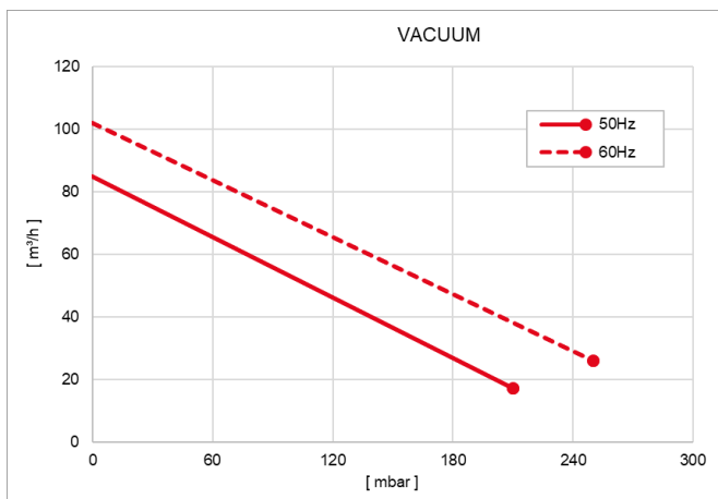
Curves refer to 1013mbar (Abs.) pression and 20°C temperature (tolerance ±10%)
